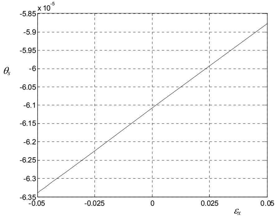
Fig. 5.21 Motion stage yaw vs. X actuator misalignment
