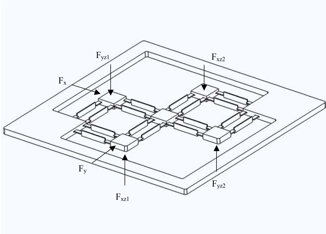
Figure 2.12 XYZ\theta_x\theta_y , Design 1
