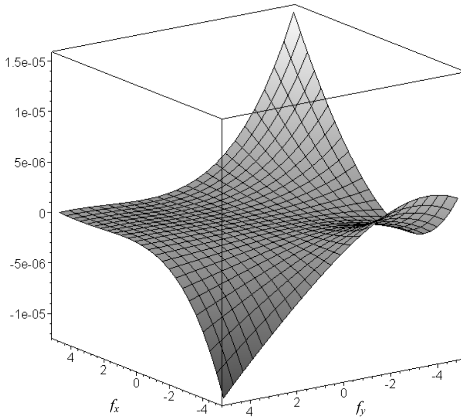
Fig. 5.32c. Motion Stage Yaw vs. X force and Y force
