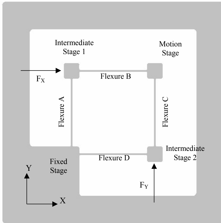
Fig. 2.6 XY Design 1
