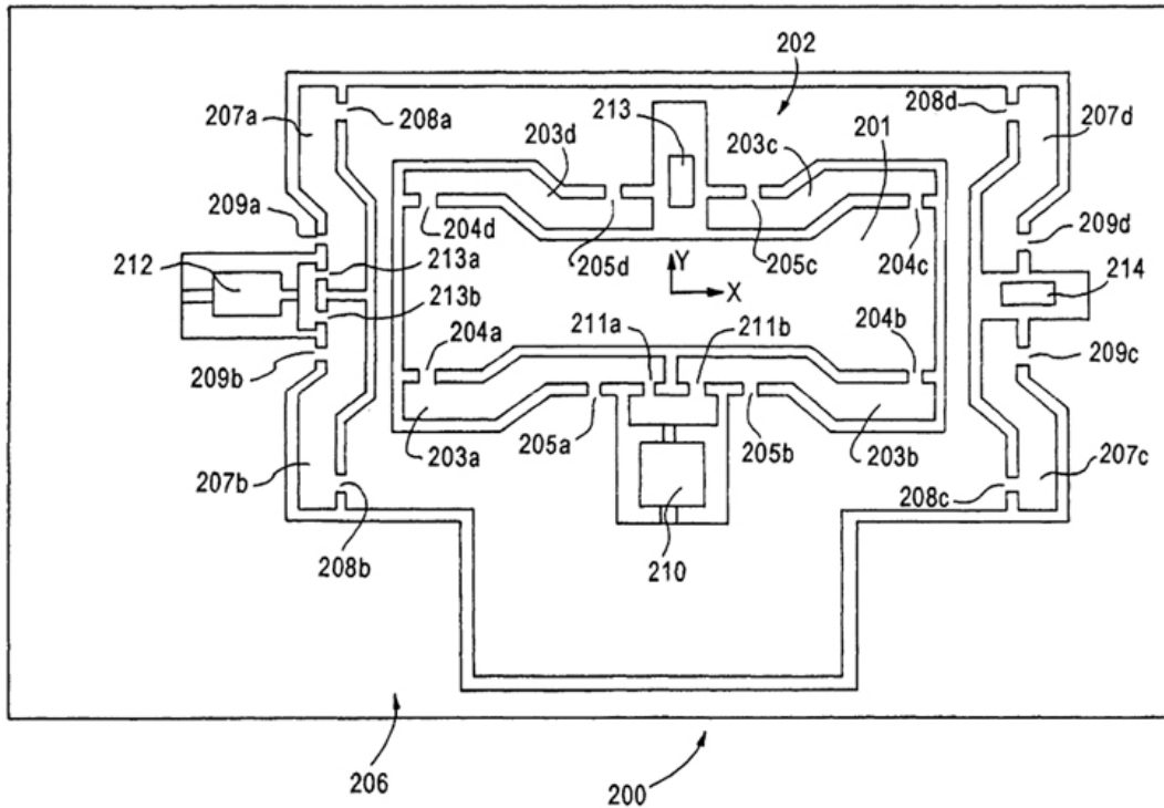
Fig.1.3 A Two DOF (X-Y) Serial Mechanism [45]
