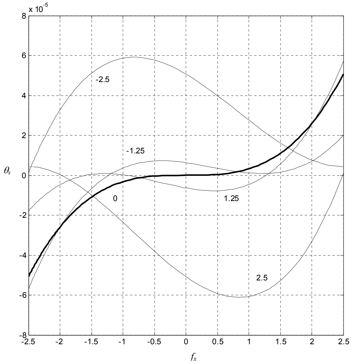
Fig. 5.19 Motion stage rotation versus f_x for different values of f_y
