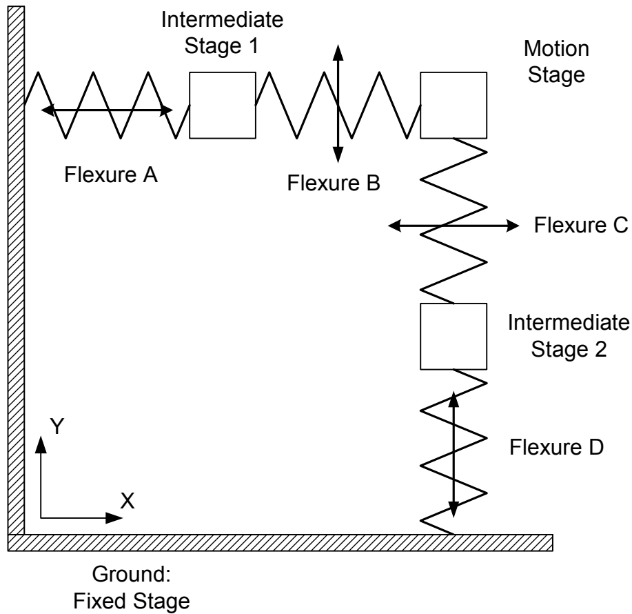
Figure 2.3 XY Flexure Mechanism Topology
