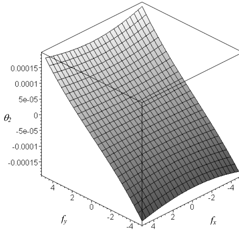
Fig5.35 Stage2 rotation versus f_x and f_y
