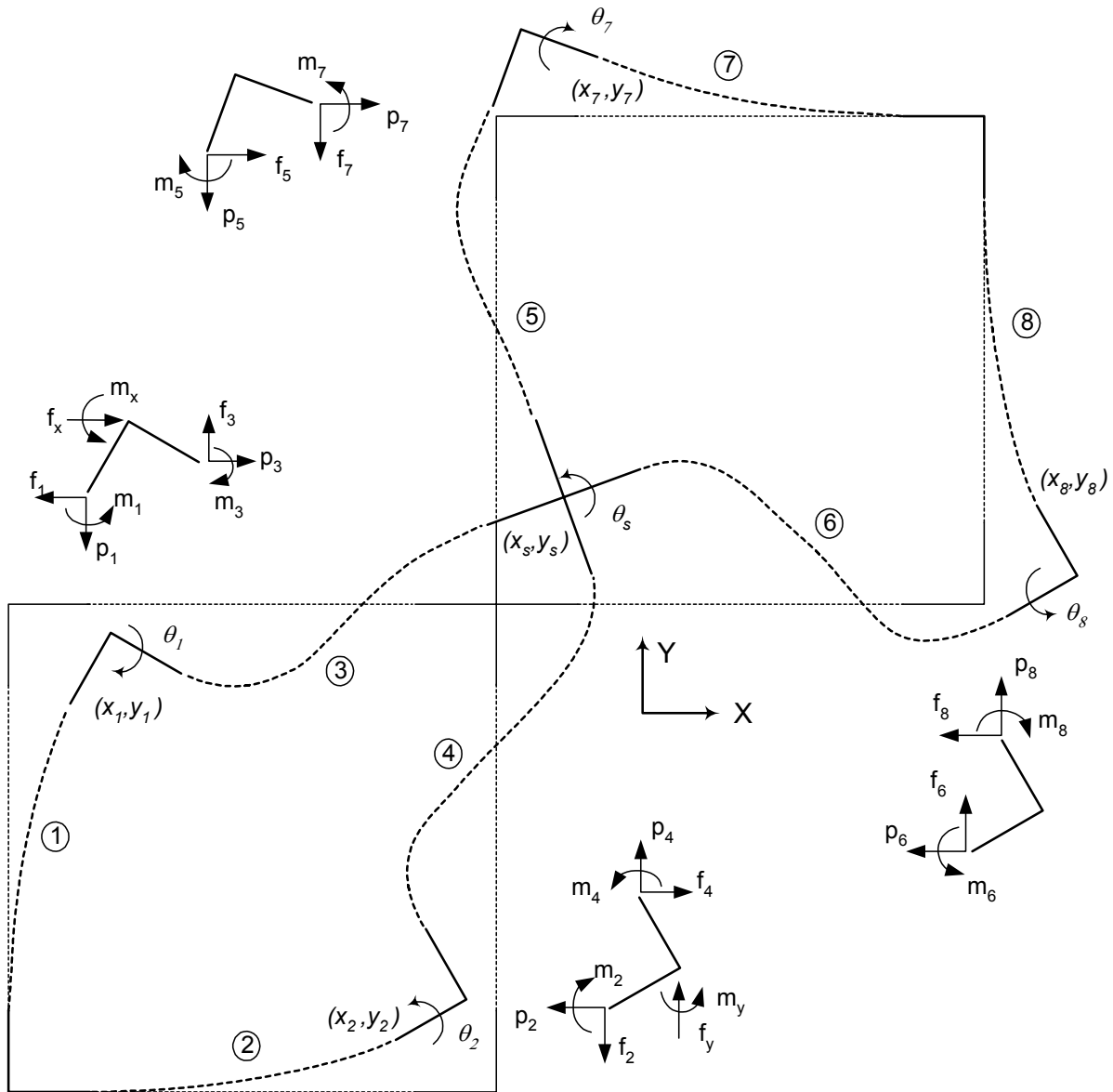
Fig. 5.10 Deformed configuration of XY Mechanism 4
