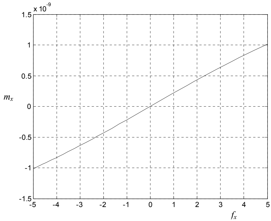
Fig. 5.26 m_x required to maintain \theta_s=0 , when f_y=m_y=0
