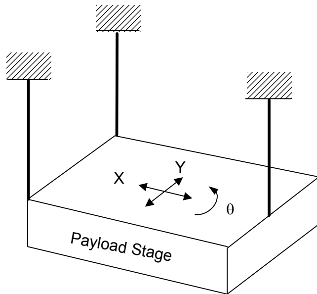
Fig. 2.1 Typical parallel kinematic XY \theta flexure mechanism
