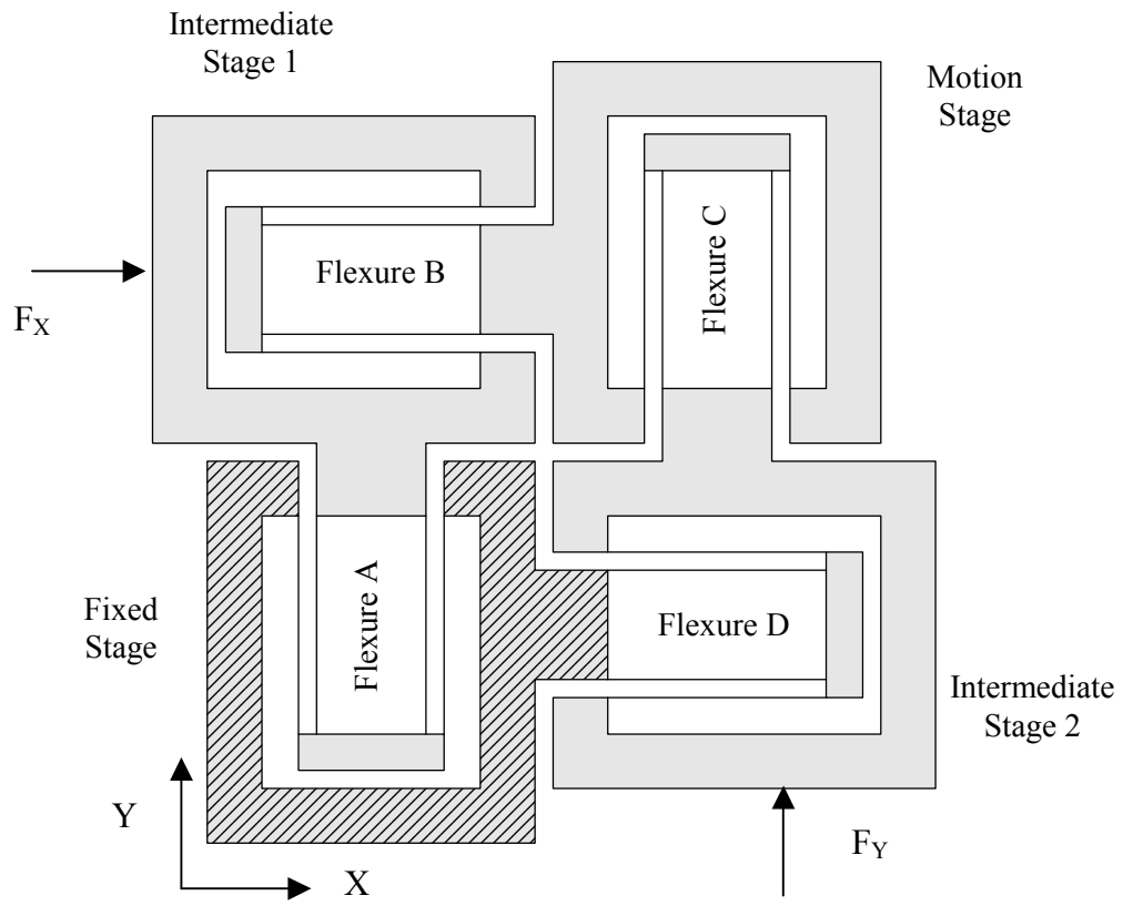
Figure 2.14 XY Design 5a and 5b
