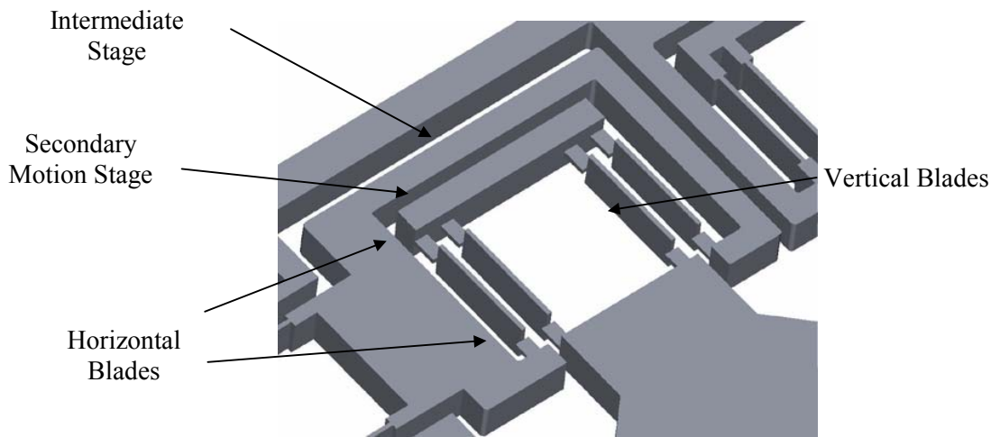
Figure 2.16 Vertical and horizontal blades produce in-plane and out-of-plane motion
