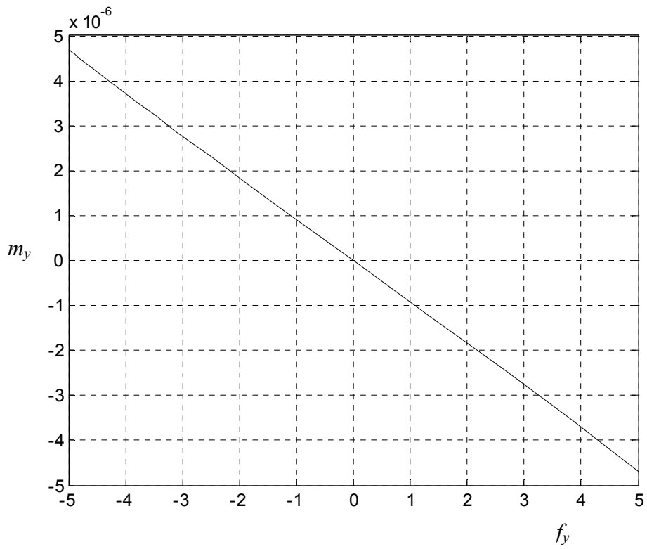
Fig. 5.27 m_y required to maintain \theta_s=0 , when f_x=m_x=0
