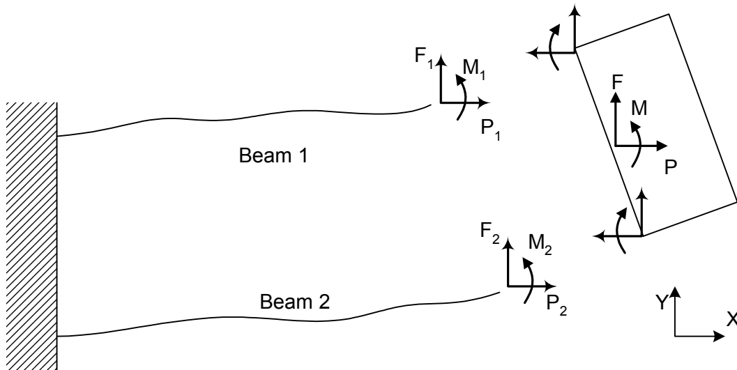
Fig. 4.2 FBD of the parallelogram flexure platform
