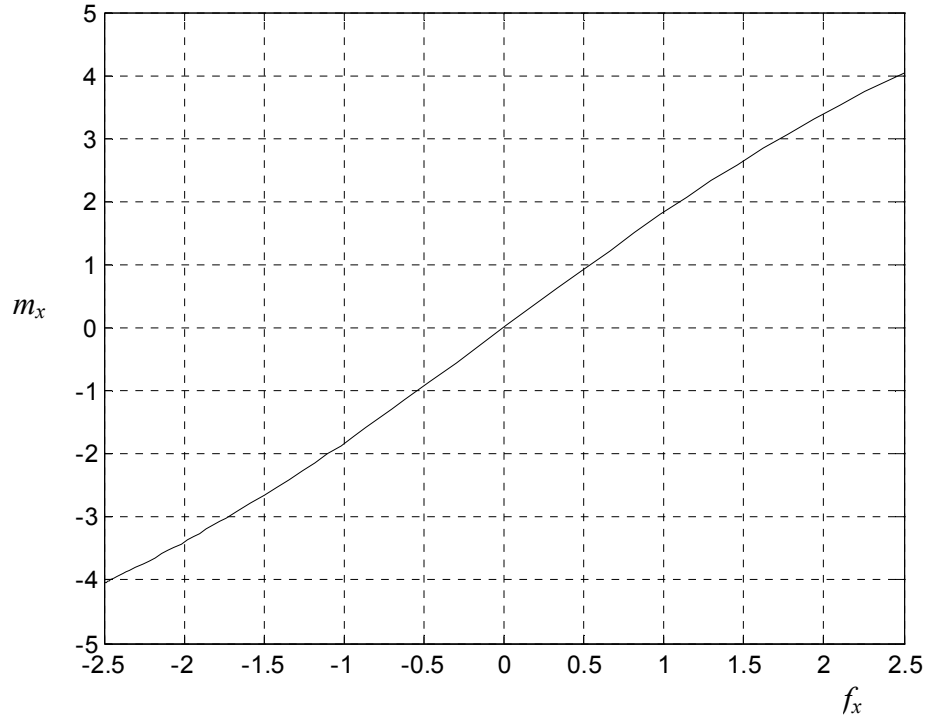
Fig. 5.17 m_x required to maintain \theta_s=0 , when f_y=m_y=0
