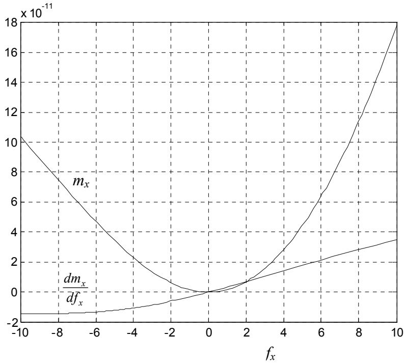
Fig. 5.11 m_x required to keep \theta_s = 0
