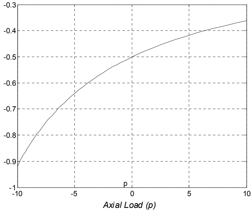
Fig. 4.5 m/f ratio required to maintain zero platform rotation
