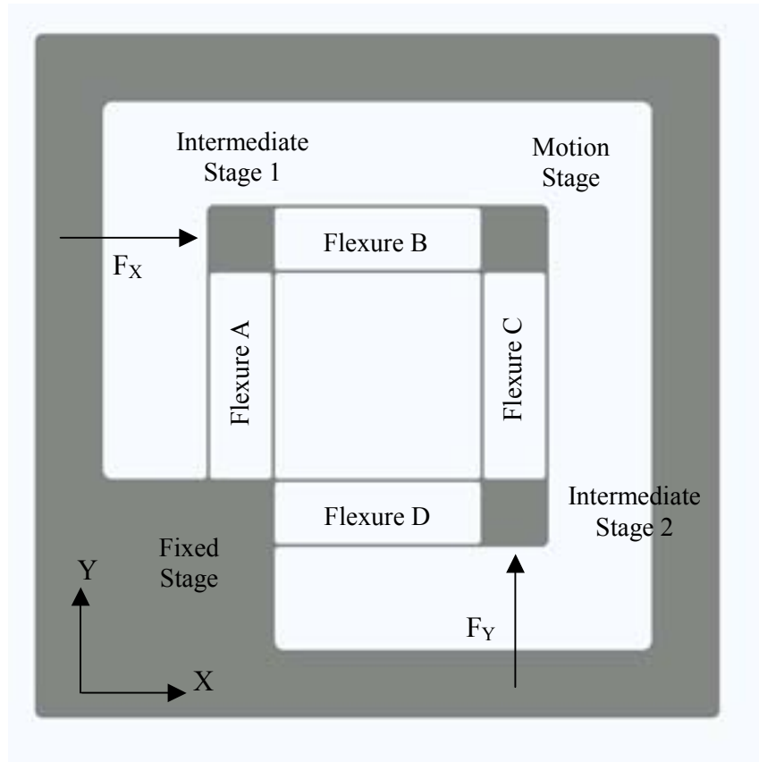
Figure 2.9 XY Design 3
