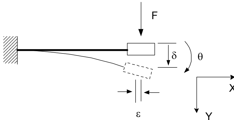
Fig. 2.5 Simple Beam
