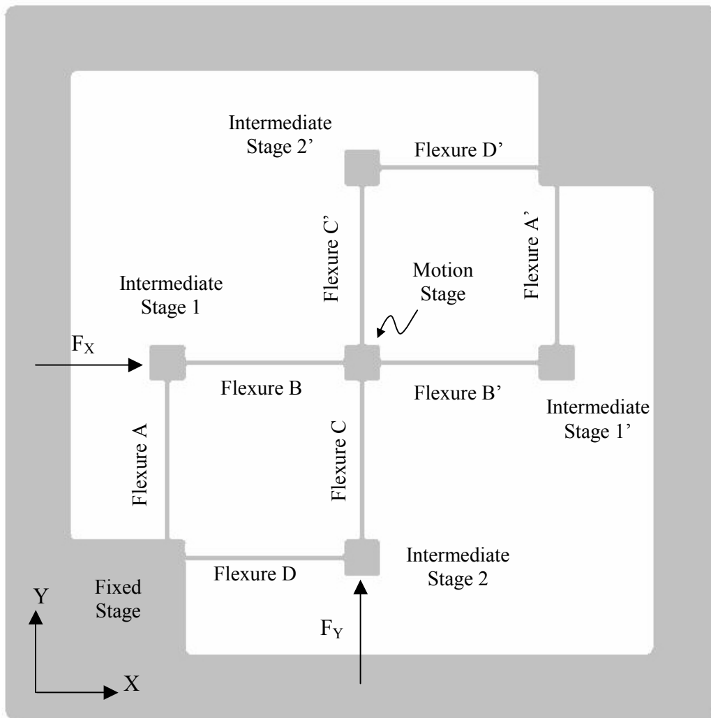
Fig. 2.7 XY Design 2
