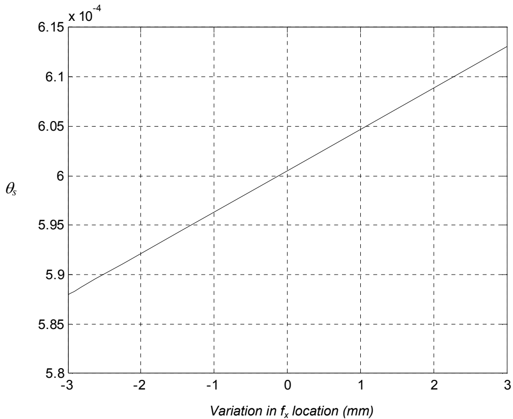
Fig. 5.8 Sensitivity of \theta_s to X force location
