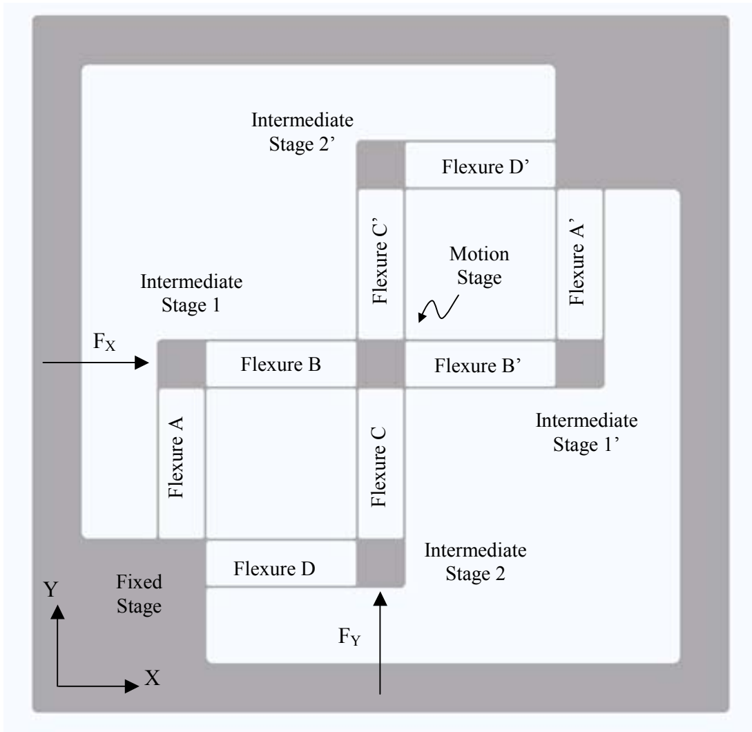
Figure 2.10 XY Design 4
