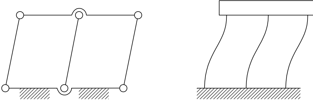
Fig. 1.2 a) Multiple parallelogram linkage mechanism b) Multiple parallelogram flexure mechanism
