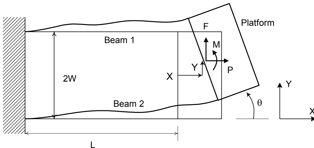
Fig. 4.1 Parallelogram Flexure
