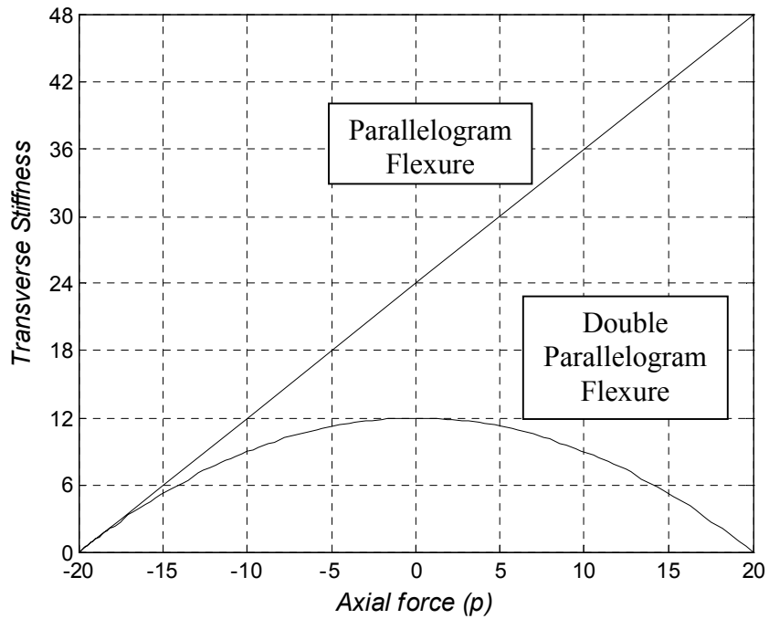
Fig. 4.10 Comparison of transverse stiffness of parallelogram and double parallelogram flexures
