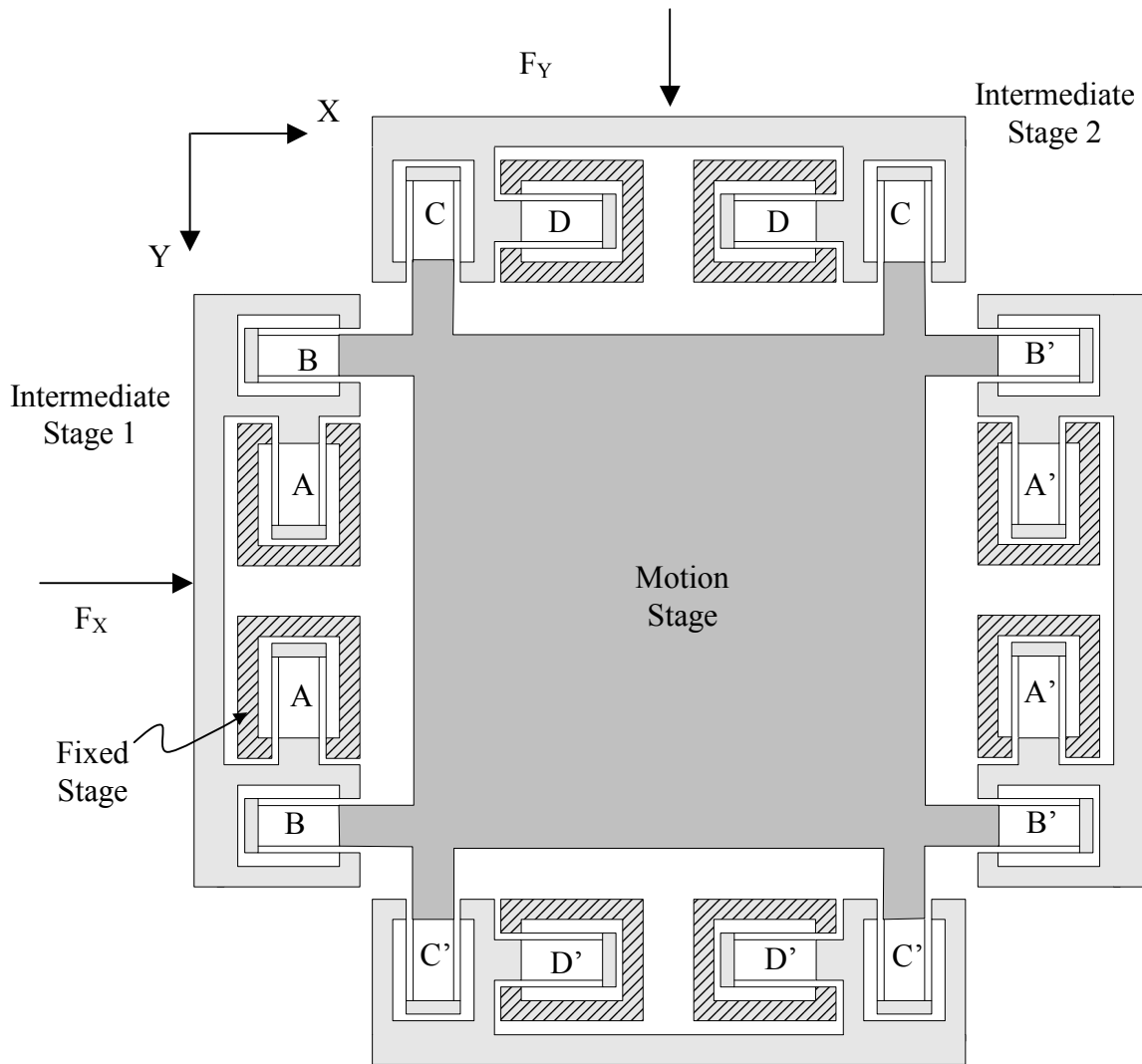
Fig. 2.16 XY Design 7
