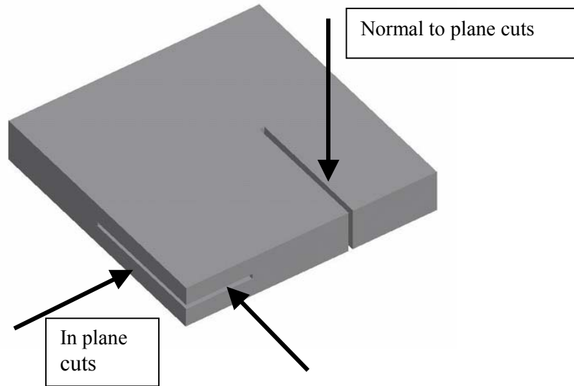
Fig 6.12 In-pane and normal to plane cuts
