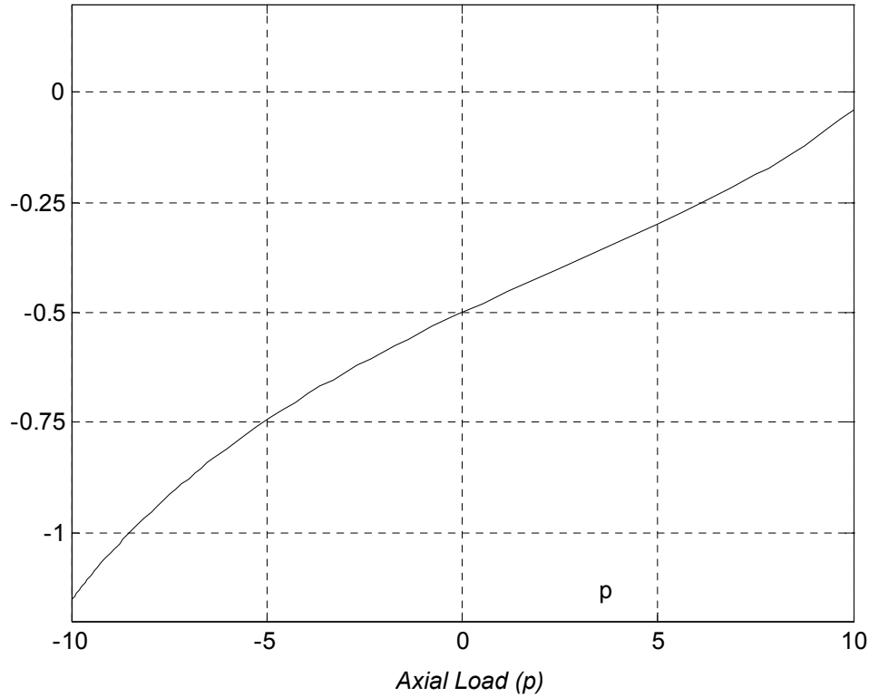
Fig. 4.12 m/f ratio required for zero platform rotation
