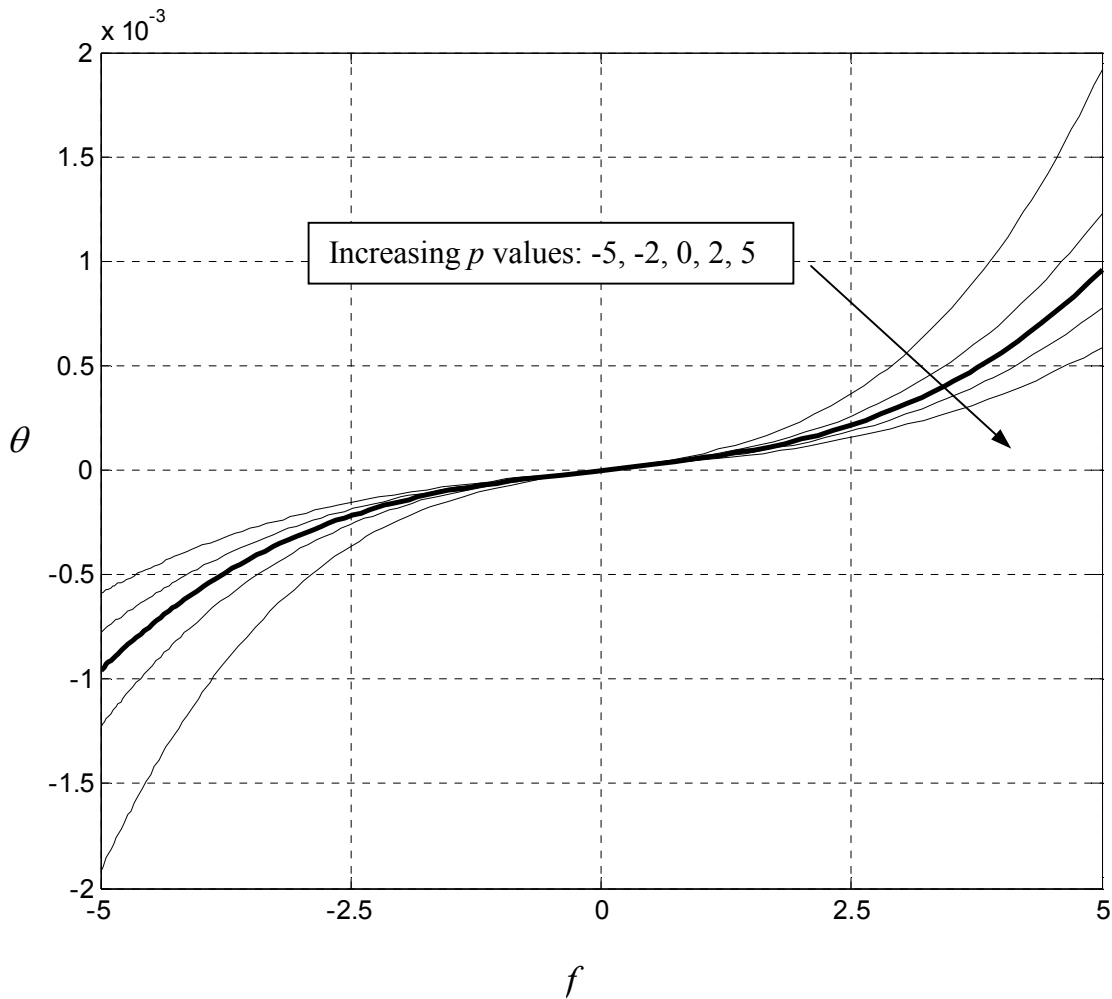
Fig. 4.4 Dependence of f - \theta relationship on the axial load p
