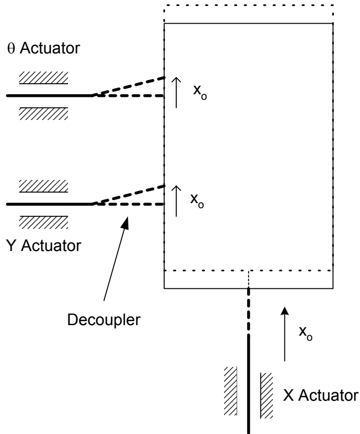
Fig. 2.2 Actuator – Stage Integration
