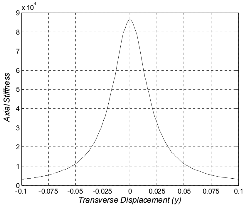
Fig. 4.13 Dependence of axial stiffness on the transverse displacement
